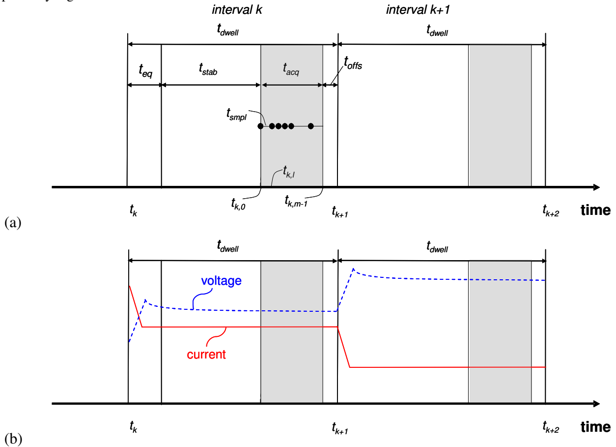
Figure 7.3: Schematic of the timeline for two consecutive set points k and k+1 of test step 3 each having a dwell time of same duration (a). The test input and output (test variables) are sampled l times at t_{k,l} ( 0 \leq l \leq m-1 ) to collect m measurements with a sampling interval of t_{smpl} during t_{acq} (see also Table 13). The principle profile of the current as a main test input and of the resulting stack voltage as a major test output are shown for the two intervals k and k+1 where the current decreases at the beginning of each interval (b). This is representative for the ramping down of the current at anyone set point k and k+1 between (inclusive) the maximum current density and the minimum current density in step 3 of the test (see also Figure 7.2).
