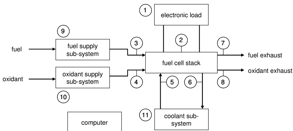
Figure 6.1: Test set-up with sub-systems and sensors and sensor locations (see also Table 8 and Table 9).
