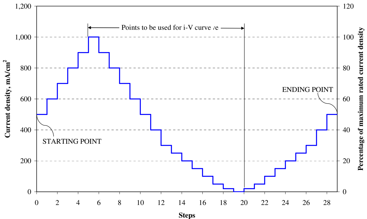
Figure 7.2 Example of one complete current density cycle with 28 steps of instantaneous changes in current according to the 15 set points k in Table 11. This cycle has a start value (starting point) and end value (ending point) at 500 mA/cm 2 and the maximum current density is 1,000 mA/cm 2 . The number of steps during the current increase from the starting point to the maximum current density and also from the minimum current density (OCV) to the ending point may be reduced to shorten the overall test duration which shall be documented in the test report.
